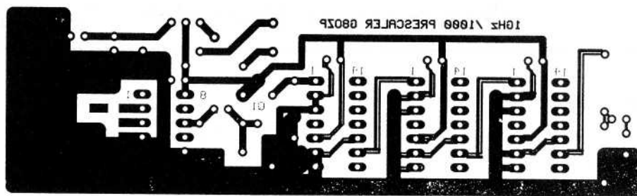
Fig.2:PCB Layout
