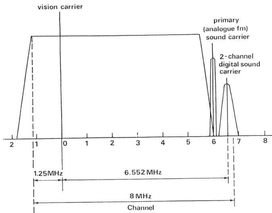
8 MHz PAL System 1 channel with additional NICAM 728 2-channel digital sound: diagrammatic representation of the frequency bands occupied by the vision and sound signals.
